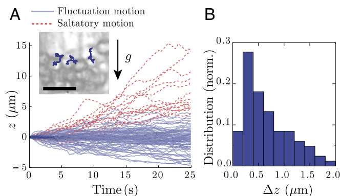
Fig. 2. Statolith agitation. (A) Vertical trajectories of n statoliths at the surface of a sedimented pile ( n = 98 ). Blue, fluctuating motion defined by \Delta z_{\text{max}} < d within the observation time window ( t = 25 s). Red, saltatory motion defined by \Delta z_{\text{max}} > d . (Inset) Picture of statoliths at the top of a sedimented pile with individual 2D trajectories drawn. (Scale bar, 10 \mu\text{m} .) (B) Measured distribution of \Delta z (SD of vertical trajectory) for the fluctuation motion ( n = 83 ).
