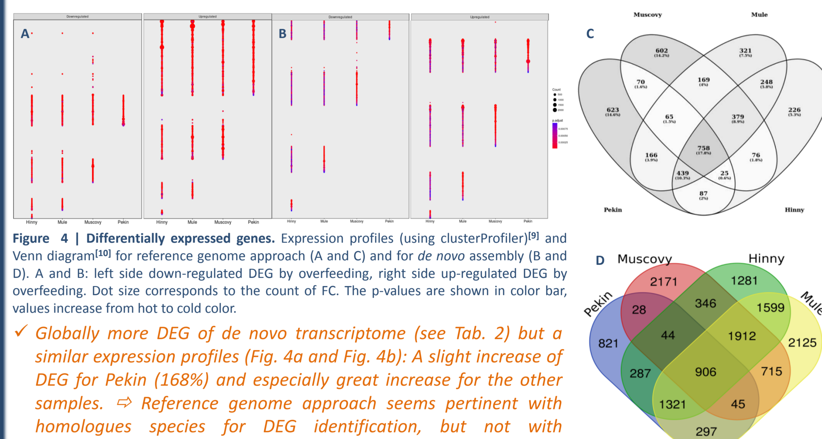
Figure 4 | Differentially expressed genes. Expression profiles (using clusterProfiler [9] ) and Venn diagram [10] for reference genome approach (A and C) and for de novo assembly (B and D). A and B: left side down-regulated DEG by overfeeding, right side up-regulated DEG by overfeeding. Dot size corresponds to the count of FC. The p-values are shown in color bar, values increase from hot to cold color.
