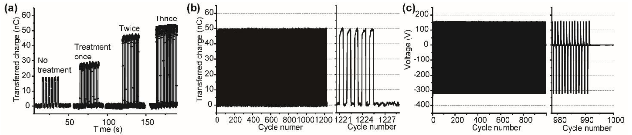
Fig. 7. (a) Increased transferred charge amount of the TENG by increasing tape treatment counts. (b) Durability of the TENG in transferred charge amount. (c) Durability of the TENG in output voltage.
