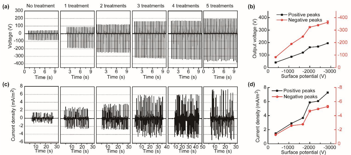
Fig. 6. Improvement of the TENG in output voltages and currents. (a) Increased output voltages of the 4 \times 4 \text{ cm}^2 sized TENG with the FEP film treated by the tape with increasing counts (from left to right: 0~5 counts). (b) Statistic results of the positive and negative voltage peak values. (c) Increased current density of the TENG with increasing treatment counts. (d) Statistic results of the positive and negative current density peak values.
