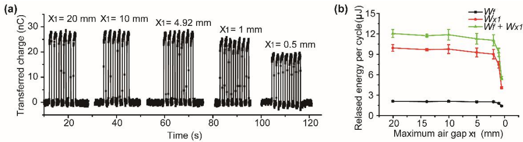
Fig. 4. (a) Measured transferred charge amounts and (b) calculated released energy per cycle from the TENG with different x_1 .
