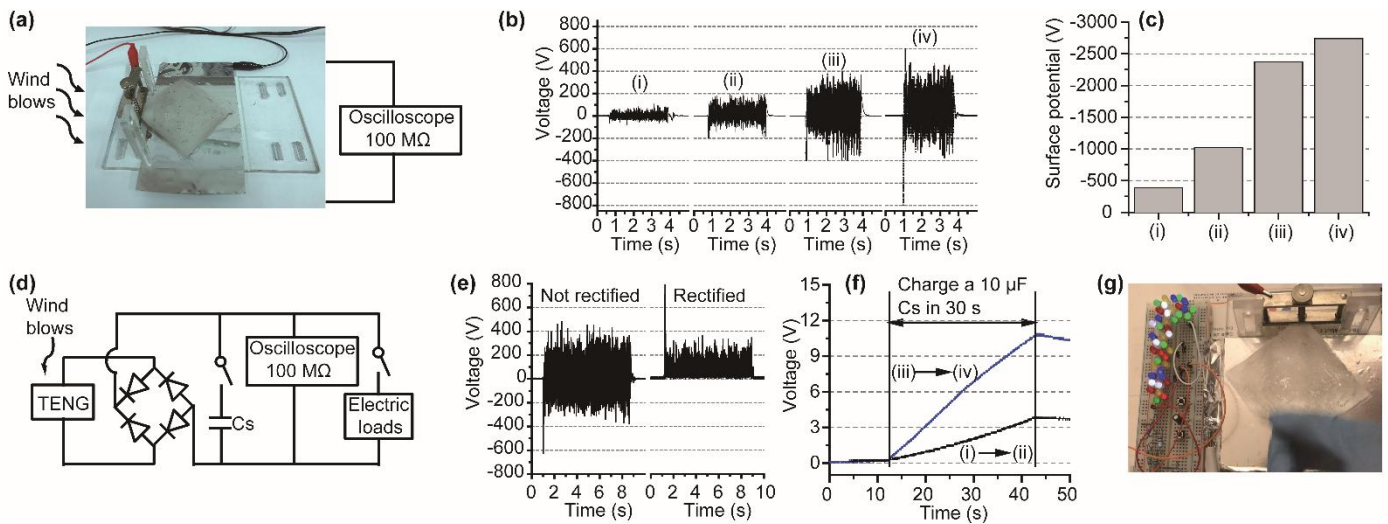
Fig. 8. Demonstrations of energy harvesting by the TENG from wind and human motions. (a) The photograph of the wind-driven TENG with an 8 cm × 8 cm sized FEP film, and the illustration of its working process. (b) Output voltages of the TENG with FEP film holding different surface potentials. (c) Measured surface potentials of the FEP film corresponding to the output voltages in (b). (d) The circuit diagram of the TENG driven by wind to charge a capacitor (Cs) or to power electric loads. (e) Output voltage of the TENG before and after rectification, driven by wind. (f) Charging curves of the Cs charged by the TENG before and after tape treatment. (g) The photograph showing that 42 LEDs were directly lighted up by the TENG when the FEP film was slightly and slowly flapped by a human hand.
