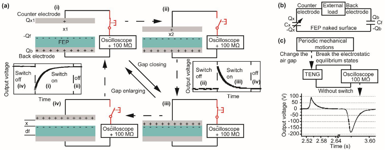
Fig. 1. Working principle of the TENG explained with the variable capacitance model. (a) The schematic of one working cycle of the FEP electret film-based gap varying TENG. (b) The equivalent circuit diagram of the capacitance model of the TENG. (c) The diagram showing the working process of the TENG and its output voltage without switch in the external circuit.
