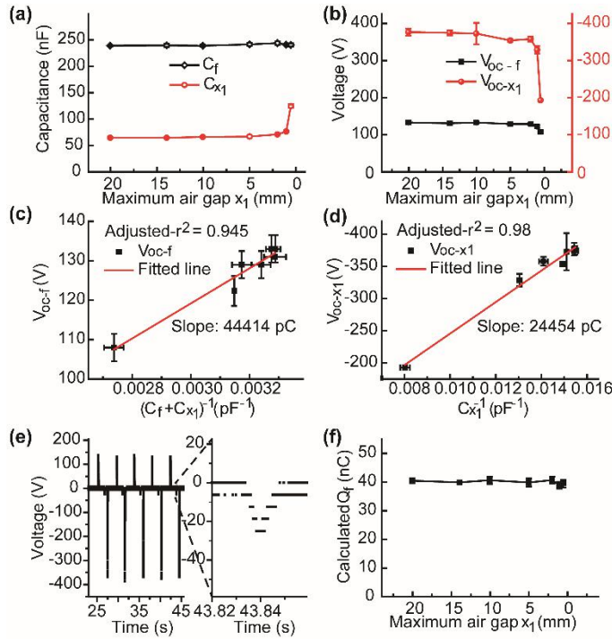
Fig. 3. Verification of the variable capacitance model. (a) Statistic results of calculated C_f and C_{x1} values with different x_1 . (b) Statistic results of calculated peak V_{oc-f} and V_{oc-x1} with different x_1 . (c) V_{oc-f} as a function of (C_f+C_{x1})^{-1} . (d) V_{oc-x1} as a function of C_{x1}^{-1} . (e) Partially enlarged view of the output voltage shows the electric leakage before V_{oc-x1} peaks. (f) Calculated Q_f with different x_1 by using V_{oc-f}(C_f+C_{x1}) .
