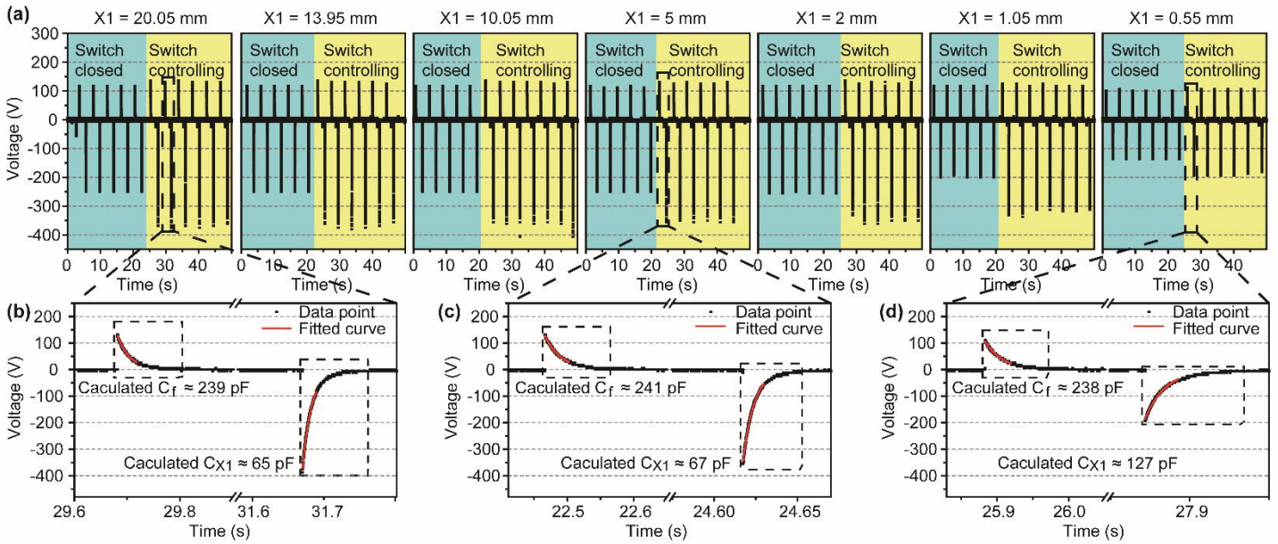
Fig. 2. The capacitor discharge fitting method for verifying the variable capacitance model. (a) The output voltages of a 4 \times 4 cm 2 sized TENG with different maximum air gap x_1 values, from left to right, x_1 varies from 20.05 mm to 0.55 mm. (b)-(d) Partially enlarged views of the output voltage peaks with x_1 set as 20.05 mm, 5 mm, and 0.55 mm respectively, and corresponding fitting results giving calculated C_f and C_{x_1} values.
