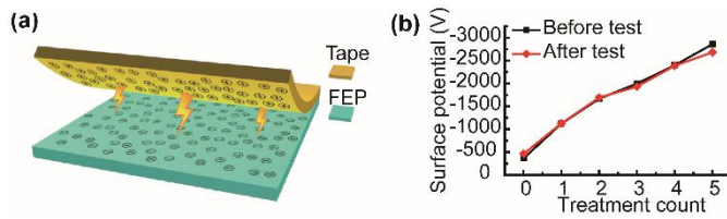
Fig. 5. Charge the FEP film with the tape-peeling method. (a) The schematic of charging the FEP film with tape. (b) Increased surface potential of the 4 \times 4 \text{ cm}^2 sized FEP film with increasing tape-peeling treatment counts, before and after the linear motor test.
