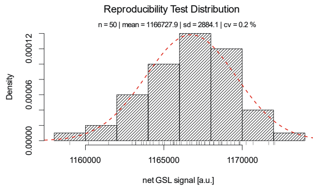
Fig. 4. Stability of the GSL emission over a series of 50 cycles consisting each of a thermal resetting, irradiation for 4 s (ca. 816 \mu Gy), GSL measurement at 70°C, a second resetting and a GSL background measurement. Results are summarised in a histogram. The intensity varies by only 0.2% ( cv ) reflecting a high system reproducibility.
