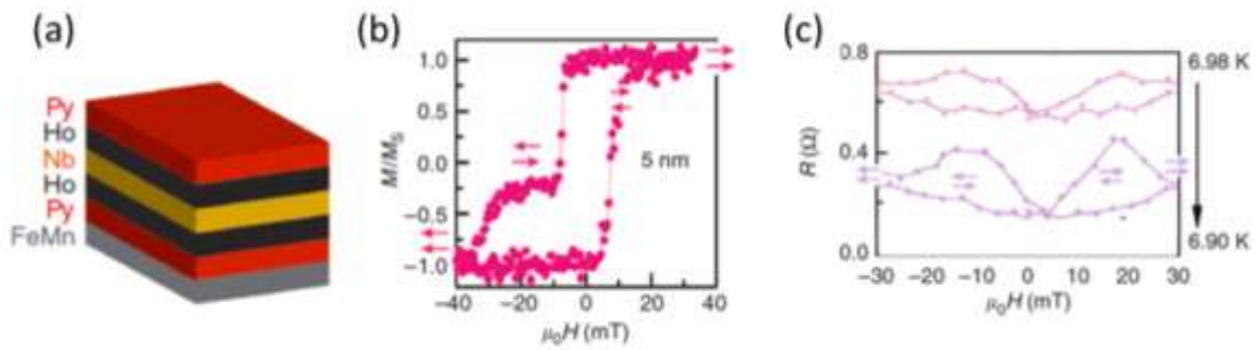
Figure 6. Superconducting spintronics. (a) Illustration of a triplet “superconducting spin valve”. The superconductor (Nb) is sandwiched between two ferromagnetic (FM) (Ho/Py bilayers). Ho is a conical magnet that behaves as a spin-mixer to generate equal-spin triplet state. (b) The hysteresis loop for a spin valve with a 5-nm-thick layer of Ho on either side of Nb shows that the exchange bias exerted by the FeMn layer on the lower Py layer, allows for parallel/antiparallel magnetization states of the Py layers. (c) The spin-valve magneto-resistance ( R ) shows hysteresis, with a resistive switching within the field range in which the Py layers magnetization is labeled antiparallel. In the case of antiparallel magnetization, some of the triplet pairs are not be able to flow from one FM electrode into the opposite one, which results in higher resistance. The effect is observed only in a narrow (few mK) temperature range across the superconducting transition ( T_c \sim 6.90 K). The curves correspond to two measurements at different temperatures within the range 6.98 to 6.90 K. Note: M , magnetization; M_s , saturation magnetization; \mu_0 , magnetic permeability of free space; H , applied magnetic field. Adapted with permission from Reference 107, copyright (2014), MacMillan Publishers Ltd.
