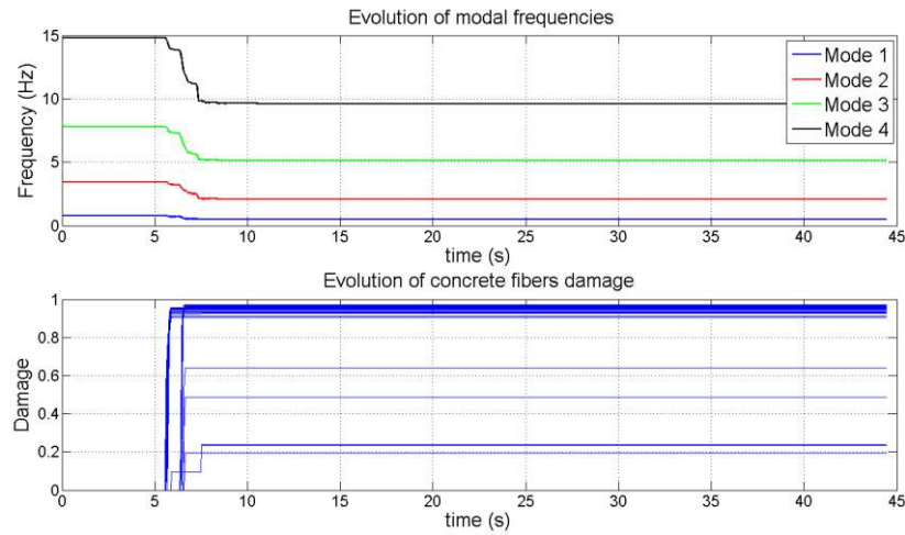
Figure 15: Evolution of damage in traction of concrete and of the modal frequencies during the non-linear dynamic simulation
