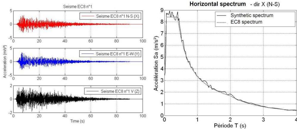
Figure 8: Set of accelerograms and spectrum of the X ones compared to the EC8 spectrum required
