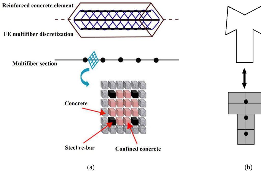
Figure 4: (a) Multifiber beam modeling, (b) Piles section discretization
