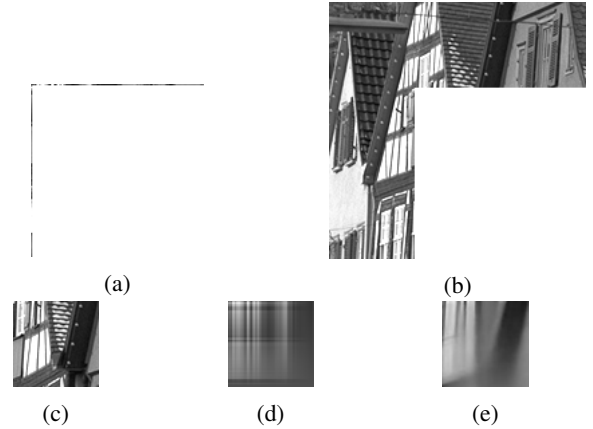
Fig. 10: Prediction of a block of size 64 \times 64 pixels via the best H.265 mode in terms of PSNR and PNNS: (a) H.265 causal neighborhood, (b) PNNS context, (c) block to be predicted, (d) predicted block via the best H.265 mode (planar) in terms of PSNR, and (e) predicted block via PNNS.
