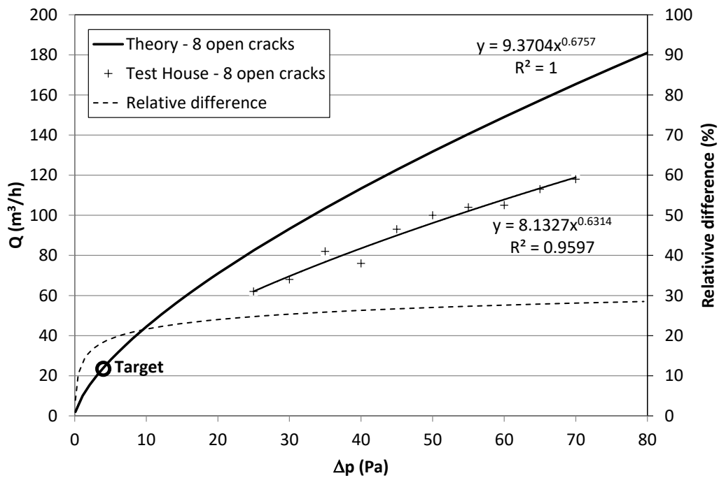
Figure 9: BAM characteristic curves obtained by in-situ measurement.
