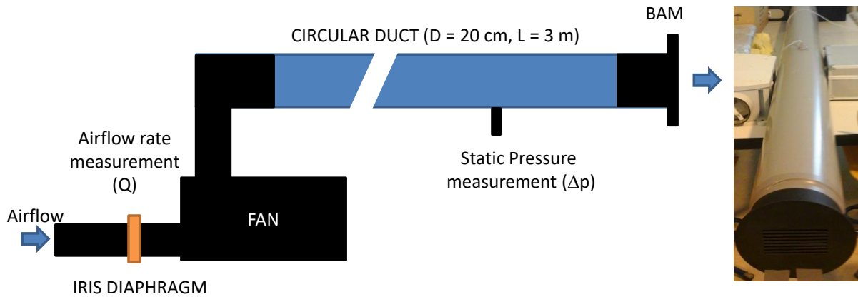
Figure 6: Experimental set-up.
