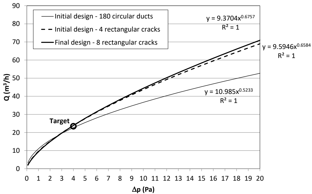
Figure 4: Characteristic curves of different BAM designs.
