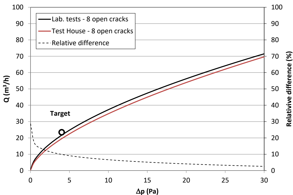
Figure 10: BAM characteristic curves obtained by lab. and in-situ measurements.
