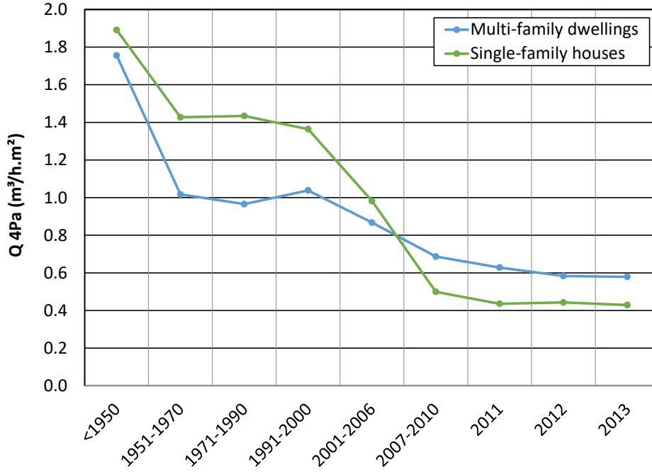
Figure 1: Evolution of the airtightness envelope measurements and their results for residential buildings in France (from Bailly et al., 2015).
