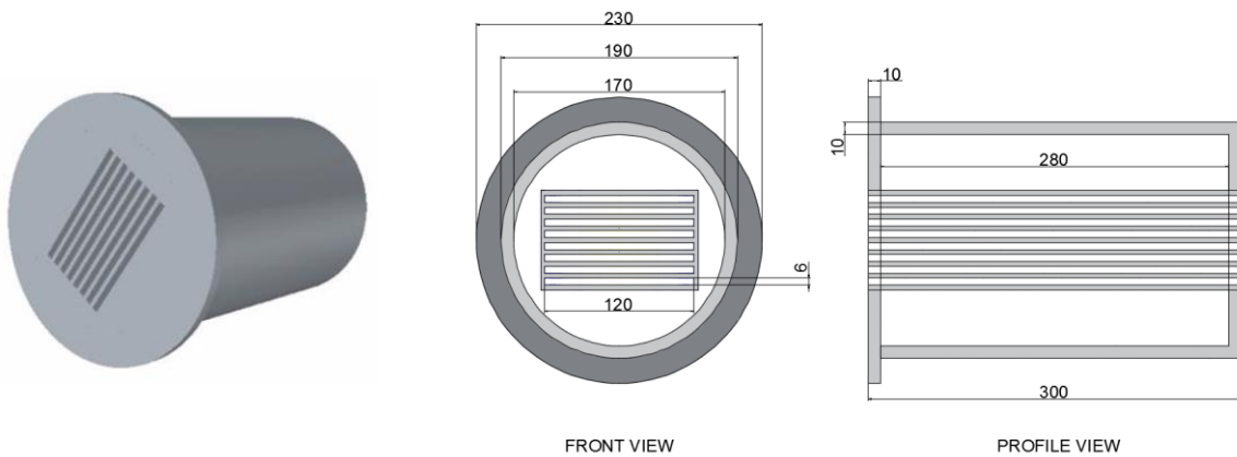
Figure 5: Final design (dimensions are in mm).
