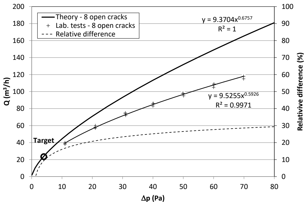
Figure 7: BAM characteristic curves obtained by measurement in the laboratory.
