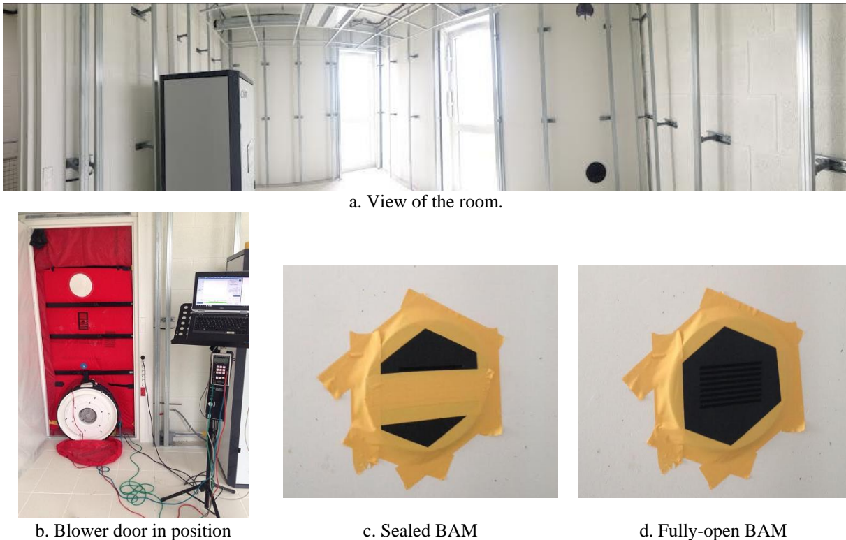
Figure 8: Experimental set-up in the test House.
