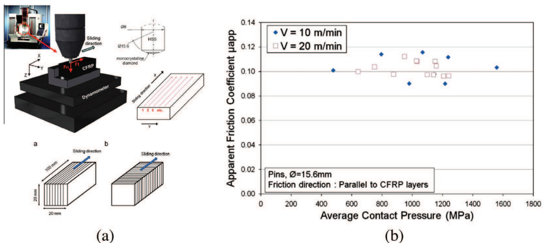
Fig. 11. Machining friction (a) and friction coefficient observed during tests (b) [26].
