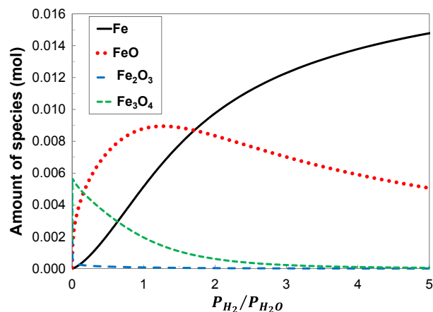
Fig. 12. Thermodynamic equilibrium of iron at 850^\circ C versus P_{H_2}/P_{H_2O} ratio.
