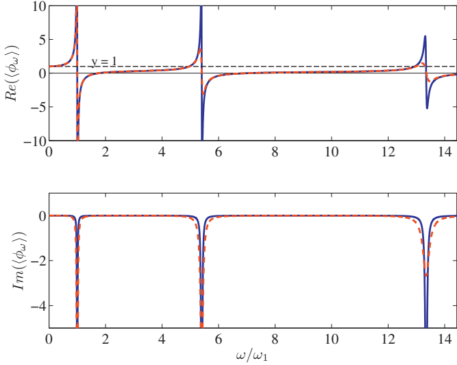
Fig. 2. Real and imaginary parts of the dimensionless apparent mass of the plate \langle\phi_\omega\rangle versus dimensionless circular frequency \omega/\omega_1 of the three first symmetric modes; with structural damping \eta = 0.5\% (—), and \eta = 2\% (---).
