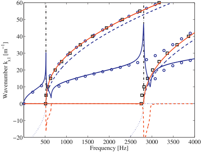
Fig. 13. Wavenumbers of the symmetric modes of propagation. Homogenized model that encompass inner resonance in bending (real part (—) and imaginary part (---)) and guided waves (real part (— · —) and imaginary part (· · ·)). CWFEM computation ( \circ ). Computation of the symmetric guided waves wavenumbers ( \square ).
