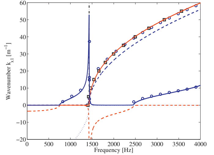
Fig. 14. Wavenumbers of the antisymmetric modes of propagation. Homogenized model that encompass inner resonance in torsion (real part (—) and imaginary part (---)) and guided waves (real part (— · —) and imaginary part (· · ·)). CWFEM computation ( \circ ). Computation of the antisymmetric guided waves wavenumbers ( \square ).
