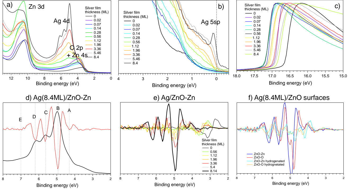
FIG. 4. UPS valence band of Ag/ZnO(0001)-Zn at 300 K as a function of Ag film thickness (1 ML = 0.235 nm): a) Evolution of the valence band showing the main contributions from the orbitals of the elements. b) Zoom on the region of the Fermi level. Notice the progressive shift of Ag 5sp metallic level toward E_F ; c) Zoom on the secondary electron cut-off. Spectra have been normalized to the maximum of intensity. Double differentiated UPS spectra : d) comparison with the actual spectrum for 8.4 ML Ag of Fig. a; e) evolution as a function of the silver thickness on ZnO(0001)-Zn and f) for a deposit of 8.4 ML on bare and hydrogenated ZnO(0001)-Zn and ZnO(0001)-O surfaces.
