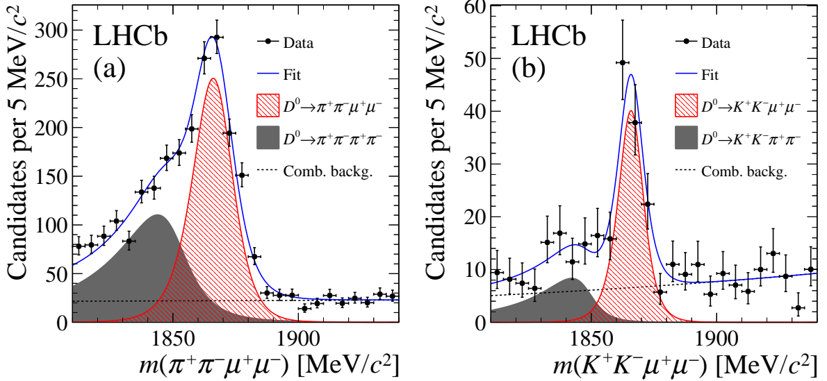
Figure 2: Distribution of m(h^+h^-\mu^+\mu^-) for (a) D^0 \rightarrow \pi^+\pi^-\mu^+\mu^- and (b) D^0 \rightarrow K^+K^-\mu^+\mu^- efficiency-weighted candidates, with fit projections overlaid.
