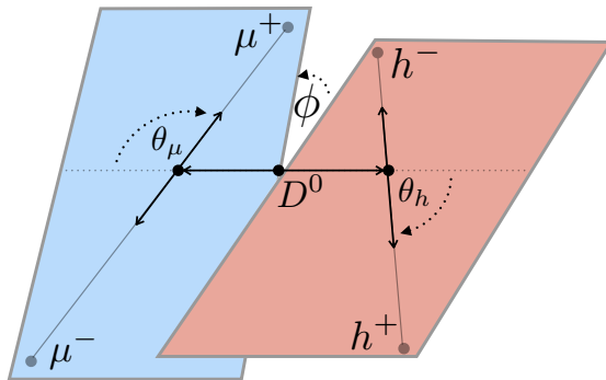
Figure 1: Diagram showing the topology of a D^0 \rightarrow h^+h^-\mu^+\mu^- decay, with the definition of the angles that are relevant for the measurement.
