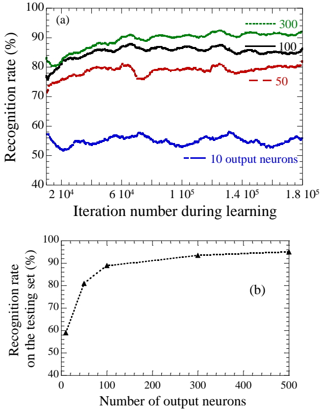
Figure 7. (a) Recognition rate during learning for simulations with different numbers of output neurons (from bottom to top: 10, 50, 100, 300). The recognition rates are running averages on 10,000 iterations. (b) Recognition rate on the test dataset as a function of the number of output neurons
