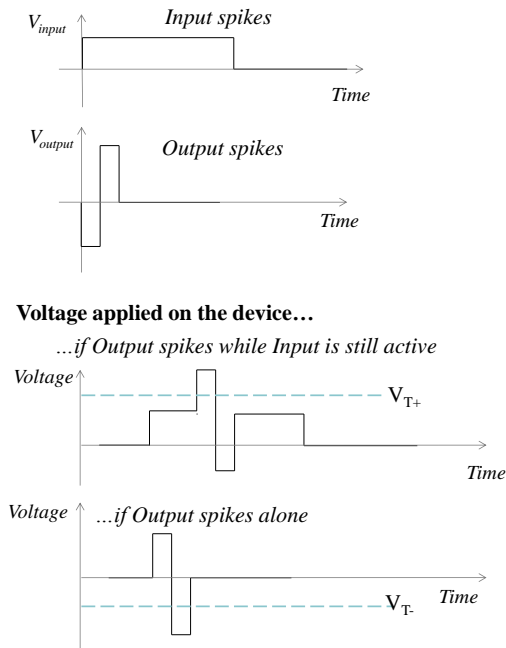
Figure 4. Pulses for simplified STDP (voltage pulses as a function of time). When an input neuron spikes, it applies an input pulse to the nanodevices to which it is connected. When an output neuron spikes it applies an output pulse to the nanodevices to which it is connected. When the voltage applied on the device (difference between the voltages applied at the two ends) reaches a memristive device threshold ( V_{T+} or V_{T-} ), its conductance is increased by a quantity \delta G_+ , or decreased by \delta G_- , respectively
