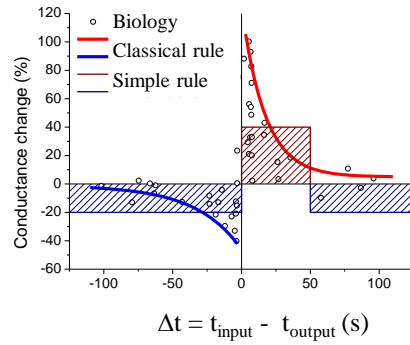
Figure 3. Our simplified STDP rule compared with the standard biological STDP rule.
