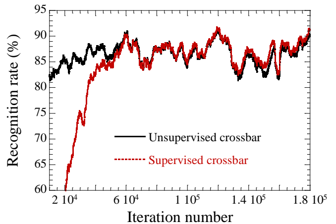
Figure 11. Two layer learning. Learning rate of the second (labeling) layer trained by variability compatible supervision (red) compared with learning of the first layer (black), as computed in the previous section. Variability of 10% on all parameters (initial conductances, \alpha_+ , \alpha_- , G_{\min} , G_{\max} )
