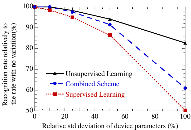
Figure 8. Robustness to devcie variation for the three schemes (unsupervised, supervised, combined). Degradation of the system’s recognition rate as a function of device variability. The variable parameters are \alpha_+ , \alpha_- , G_{min} , G_{max} .
