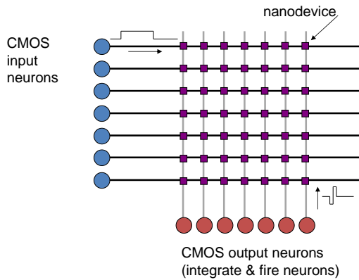
Figure 1. General architecture for the unsupervised case
