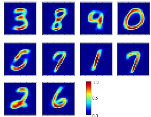
Figure 6. Conductances learned in a simulation with 10 output neurons. Red is maximum conductance ( G_{\max} ), blue is minimum conductance ( G_{\min} ).
