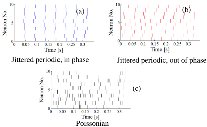
Figure 2. Illustration of the three stimulus coding schemes (a), (b), (c). Stimulus spikes timing for ten input neurons with the same pixel value in the three schemes. All three coding schemes give identical performance in terms of recognition rate. (b) is used for simulations presented in the paper.
