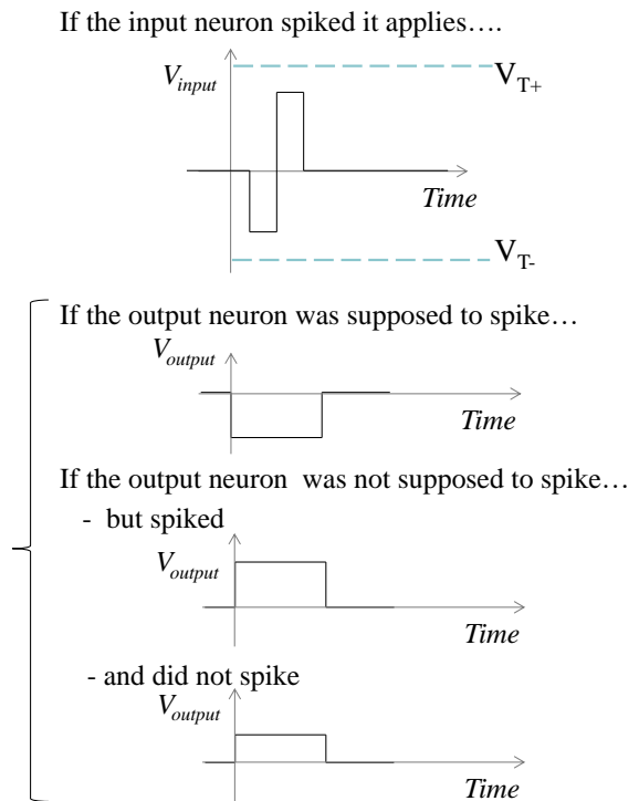
Figure 9. Voltage pulses used for supervised learning (voltage pulses as a function of time).
