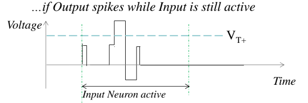
Figure 5. Low power variation of the pulses of Figure 4.
