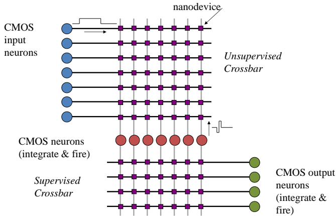
Figure 10. Architecture combining unsupervised and supervised crossbar
