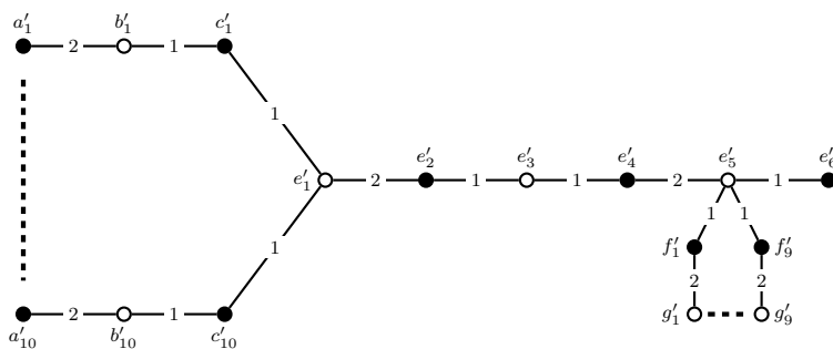
Figure 3: An extension for the initiating gadget, and the way a neighbour-sum-distinguishing [2]-edge-weighting is propagated towards e'_6 (neglecting e'_6 ). Vertices e'_1 and e'_5 are supposed to have degree 11, their neighbours being e'_2, c'_1, \dots, c'_{10} and e'_4, e'_6, f'_1, \dots, f'_9 , respectively.
