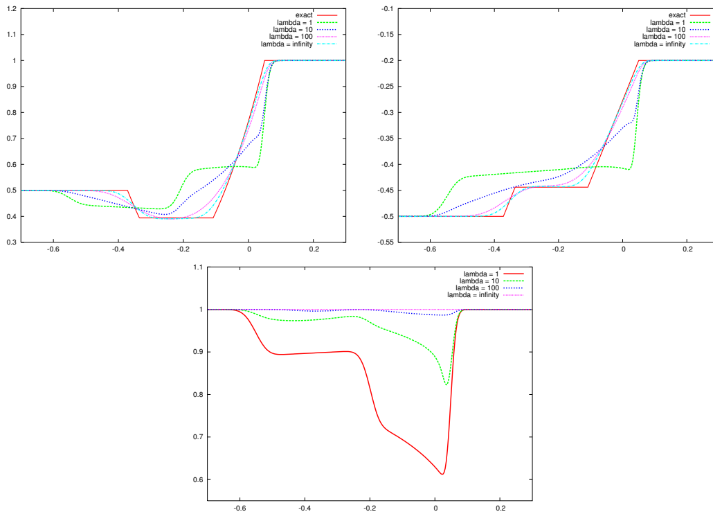
Figure 2: Test 2 : \rho (Left), u (middle) and \rho \mathcal{T} (Right) at time 0.5
