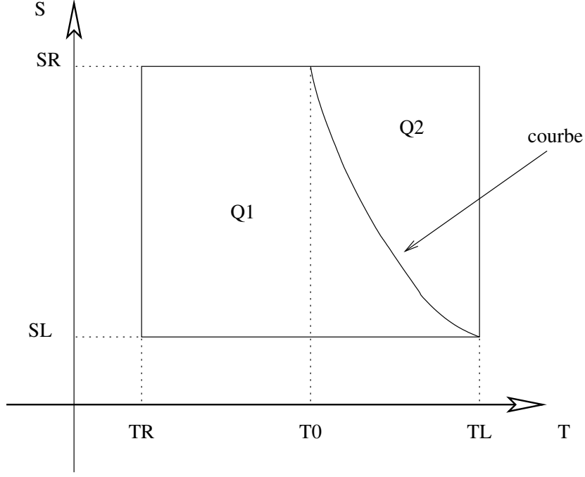
Figure 4: The square Q = [\tau_r, \tau_\ell] \times [S_\ell, S_r] , and the subsets Q_1, Q_2 .
