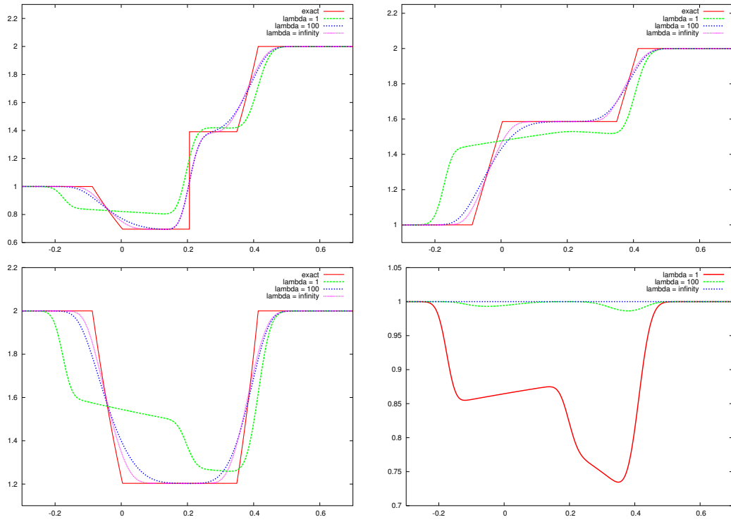
Figure 6: Test 5 : \rho (left top), u (right top), p (left bottom) and \rho\mathcal{S} (right bottom) at time 0.13
