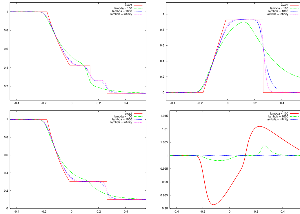
Figure 7: Test 6 : \rho (left top), u (right top), p (left bottom) and \rho \mathcal{S} (right bottom) at time 0.15
