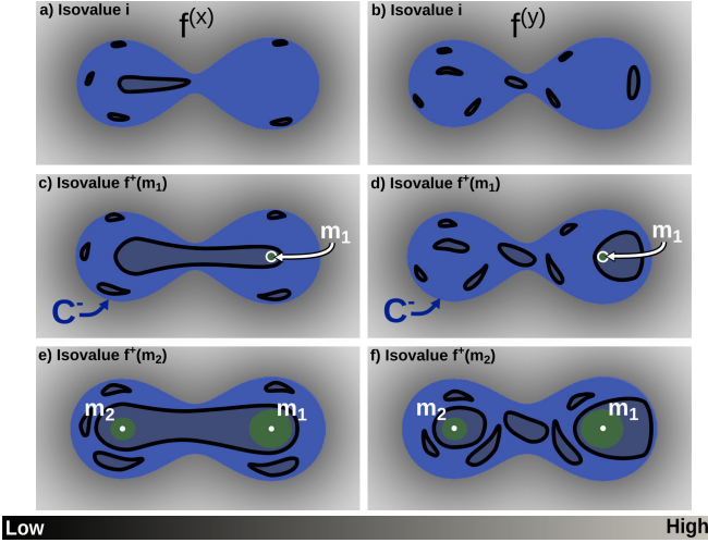
Fig. 6. Sub-level sets of f^- (blue) and f^+ (green) at three different isovalues i < f^+(m_1) < f^+(m_2) with m_1 and m_2 being minima of f^+ . The sub-level set components C^x and C^y of two ensemble members f^{(x)} (left) and f^{(y)} (right) are shown in gray.
