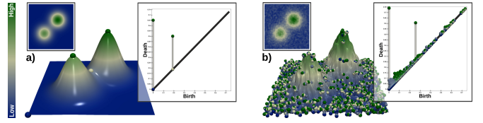
Fig. 2. Critical points (spheres, dark blue: minima, dark green: maxima, other: saddles) and persistence diagrams of a clean (a) and noisy (b) 2D scalar field. From left to right: original 2D data, 3D terrain representation, persistence diagram. The diagrams clearly exhibit in both cases two large pairs, corresponding to the main hills. In the noisy diagram (b), small bars near the diagonal correspond to noisy features in the data.
