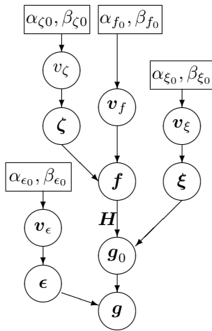
Fig. 1. Graphical representations of the proposed model.
