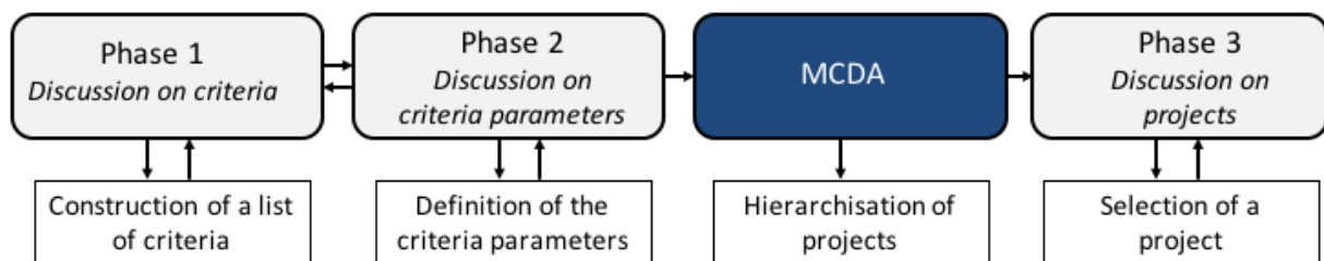
Figure 5: A decision structuring model
