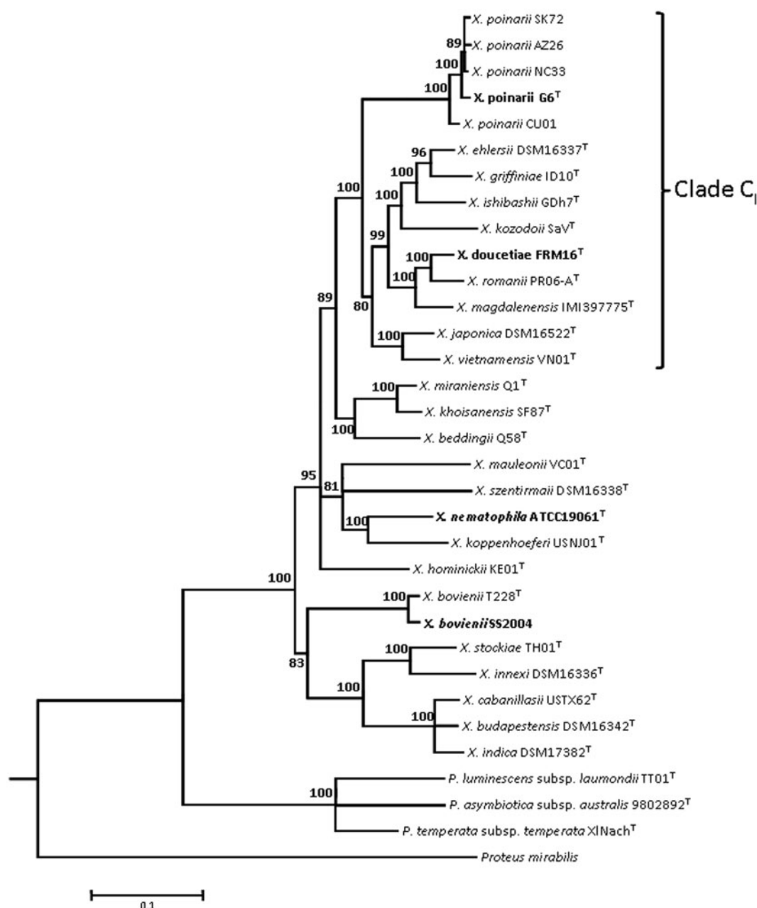
FIG. 1. —Maximum-likelihood phylogenetic tree showing the positions of Xenorhabdus poinarrii strains within the genus Xenorhabdus . The analysis is based on five concatenated protein-coding sequences ( recA , gyrB , dnaN , gltX , and infB ). It was carried out with the GTR model of substitution, with a gamma-distributed rate heterogeneity and a proportion of invariant sites. Photorhabdus and Proteus sequences were used as outgroups. Bootstrap values (Felsenstein 1988) of more than 80% (from 100 replicates) are indicated at the nodes. Clade C 1 , which includes all the X. poinarrii strains, is as previously described (Tailliez et al. 2010). The names of strains for which genomes have previously been sequenced or were sequenced in this study are indicated in bold italic and bold normal typescript, respectively. Bar: 10% divergence.
