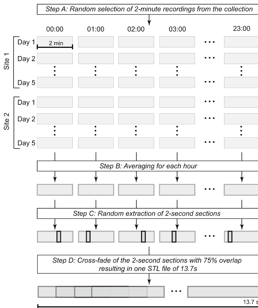
Fig. 2 Diagram of Sonic Timelapse computation. Grey rectangles, arrows, and sentences represent acoustic recordings, directions of transformation or computation, and descriptions of each computational step, respectively. The STL length is 13.7 s instead of 13.5 s due to Max/MSP program settings
