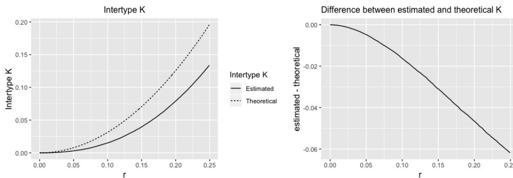
Figure 3: Example of intertype K function and its theoretical value in the homogeneous situation for Chess simulated example. Left : Intertype K -functions. Right : Difference between estimated and theoretical intertype K -functions.
