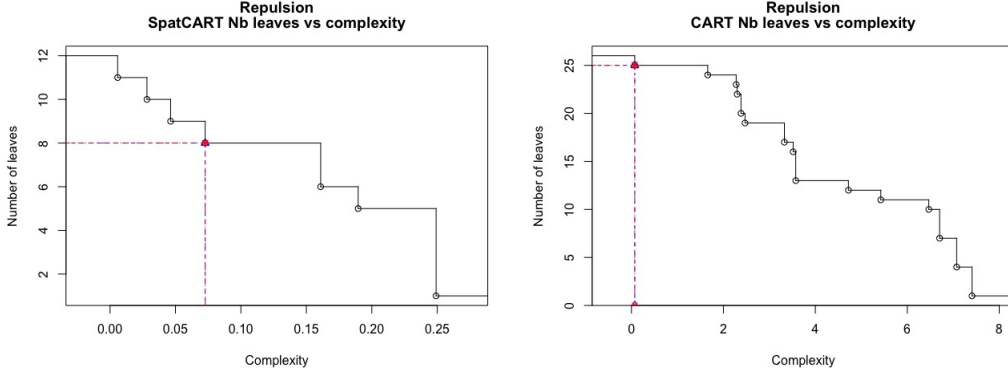
Figure 8: Behavior of number of leaves versus complexity for SpatCART and CART on Locally repulsive data set, with initial resolution r_0 smaller than the locally repulsion scale r = 0.05 . For each case, \triangle represents the tree selected via the modified largest jump method, while \diamond represents the tree selected via the largest plateau method.
