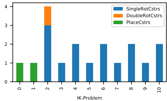
Ex1-Tree: Number of constraints
