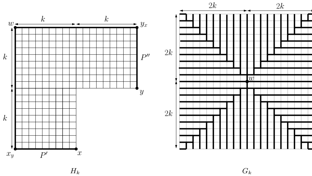
Figure 2 In H_k , \rho_{w,T} = d(x_y, y_x) = 4\delta(H_k) , showing that the inequality \rho \leq 4\delta is tight in the proof of Theorem 7. In G_k , \rho_{w,T} \leq 2k = \frac{1}{2}\delta(G_k) , showing that (up to an additive factor of 1) the inequality \delta \leq 2\rho + 1 is tight in the proof of Theorem 7.
