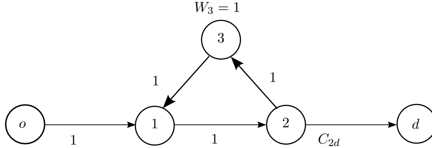
Figure 6: Instance of WTDSPP with a cyclic solution.
