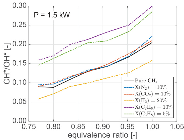
Figure 10. CH^*/OH^* vs. equivalence ratio for different fuel blend compositions.
