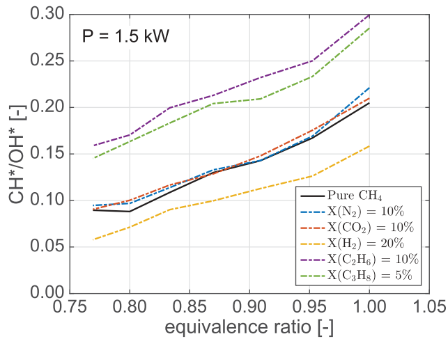
Figure 10. CH^*/OH^* vs. equivalence ratio for different fuel blend compositions.
