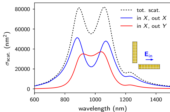
Figure 14: Polarization filtered scattering spectra from symmetric L-shaped plasmonic antenna (arm length L = 210 nm, width and height W = H = 45 nm). A sketch of the geometry is shown as inset. The total scattering (dashed black line) as well as the X and Y polarization filtered scattering contributions (blue and red, respectively) are shown.
