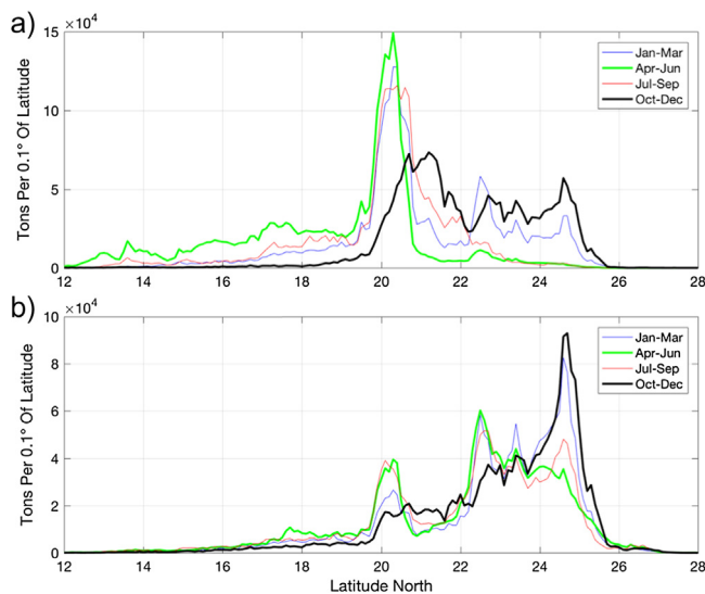
Fig. 8. (a) Mean latitudinal distribution of the population per season (blue = quarter 1, green = quarter 2, red = quarter 3, black = quarter top) obtained from model Simulation #2 (see Table 1), (b) a simulation with same parameters as Simulation #2 but in which the individuals' advection term was removed, i.e. , the only fish movement is due to swimming behavior. For each 0.1° of latitude, the biomass present on the continental shelf was sum. (For interpretation of the references to color in this figure legend, the reader is referred to the web version of this article.)
