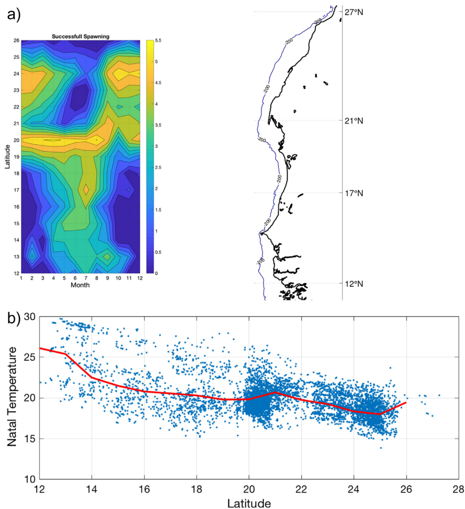
Fig. 6. (a) Spatio-temporal pattern of successful reproduction. The color bar corresponds to the number of recruited super-individuals (logarithmic scale). (b) Mean and standard deviation of sea surface temperature when successful reproduction occurs, according to latitude. Depending on the latitude, the successful reproduction mainly occurs during the first semester (south of 18°N), the second semester (north of 21°N) or year-round (from 18°N to 21°N), which explains the largest variability found at 19°N. (For interpretation of the references to color in this figure legend, the reader is referred to the web version of this article.)
