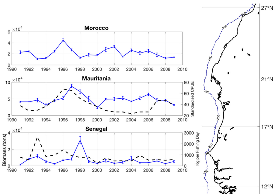
Fig. 3. Interannual fluctuations of round sardinella biomass emerging from the model (solid blue line) and comparison with field data (black dashed line). The model biomass series is computed as the yearly average biomass of fish > 12 cm located over the continental shelf of each country. The model time series presented is obtained from the mean of three repeated Simulation #2 runs with different initial conditions (see Table 1); the error bars correspond to the standard deviation between these three simulations. Model outputs are compared with (b) CPUE calculated by Braham et al. (2014) in Mauritania (IMROP), and (c) CPUE in Senegal (CRODT). No CPUE data were available for the Morocco area. (For interpretation of the references to color in this figure legend, the reader is referred to the web version of this article.)
