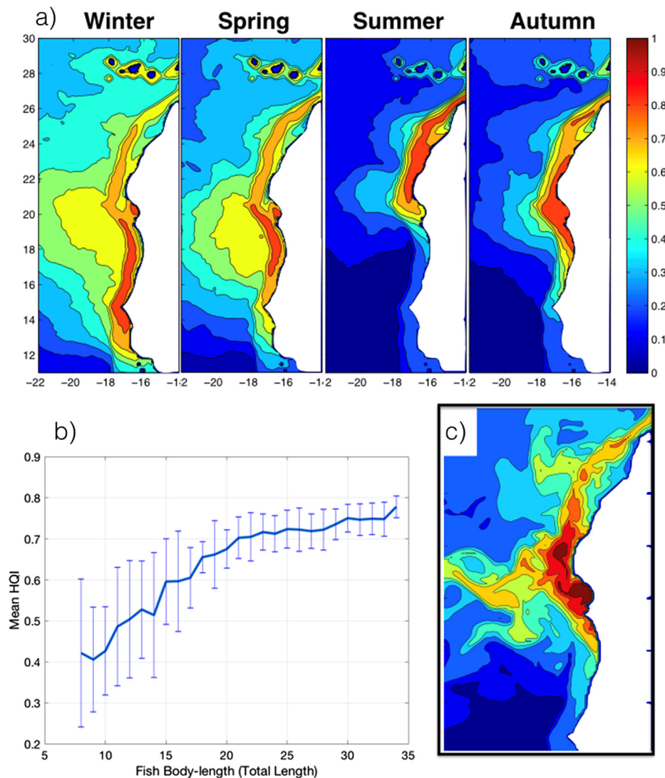
Fig. 7. Mean distribution of Habitat Quality Index for each season ( T_{pref} = 21\text{ }^{\circ}\text{C} ) (a), relationship between fish length and their ability to target high HQI (b), and a snapshot of the HQI distribution in August showing the patchy nature of HQI (c). (For interpretation of the references to color in this figure legend, the reader is referred to the web version of this article.)
