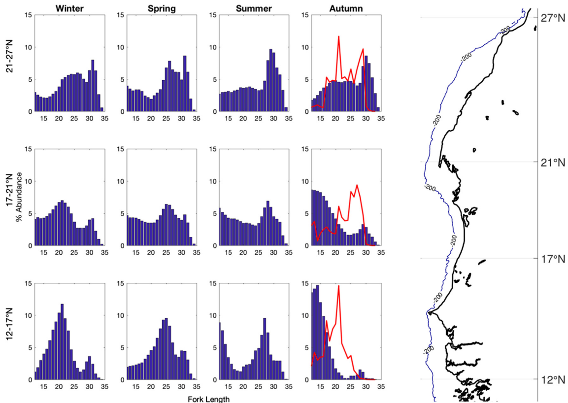
Fig. 5. Simulated fish length frequency by 1 cm class (fork length, cm) averaged over the period 1996–2004, by season and by area: Western Sahara (21–27°N), Mauritania (17–21°N) and Senegal-Gambia (12–17°N). For each area/season, the length frequency was based on the length of the fish represented by the super-individuals (SIs) weighted by the number of fish they represented ( i.e. , their worth). Seasonal variabilities are in line with fisheries data in Mauritania and Senegal (see text for details), while the increasing average size of round Sardinella from south to north is in line with average observations by the 1996–2004 Nansen scientific survey (the red lines in the autumn, see text for references). (For interpretation of the references to color in this figure legend, the reader is referred to the web version of this article.)
