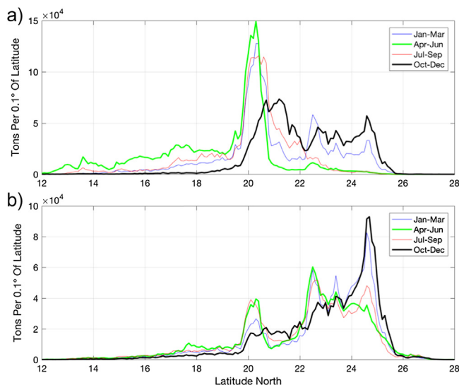
Fig. 8. (a) Mean latitudinal distribution of the population per season (blue = quarter 1, green = quarter 2, red = quarter 3, black = quarter top) obtained from model Simulation #2 (see Table 1), (b) a simulation with same parameters as Simulation #2 but in which the individuals' advection term was removed, i.e. , the only fish movement is due to swimming behavior. For each 0.1^\circ of latitude, the biomass present on the continental shelf was sum. (For interpretation of the references to color in this figure legend, the reader is referred to the web version of this article.)
