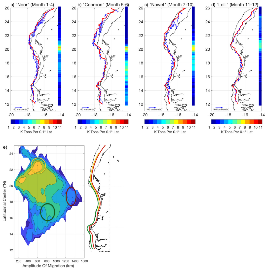
Fig. 9. Round sardinella populations traits emerging from model simulations. (a-d) Seasonal variability in spatial distribution, corresponding to the Senegalese fishing seasons; arrows show average movements (direction and intensity). The terms Noor, Cooroon, Nawet and Lolli are Senegalese terms referring to the fishing seasons and are explained in the text of the paper. The vertical color bar indicates fish biomass density (1000 Tons per 0.1^\circ latitude). The thick red line highlights the limit of the offshore extent (80% of the biomass being inshore of that limit), and the black dashed line is the 200 m isobath. (e) Distribution of migration routes (for individuals older than 12-months at the end of the year). The color scale indicates the number of individuals (color scale not shown, increasing from blue to yellow). The circled areas' migratory routes are shown on the adjacent map. (Simulation #2, cf. Supplementary Table 3). (For interpretation of the references to color in this figure legend, the reader is referred to the web version of this article.)
