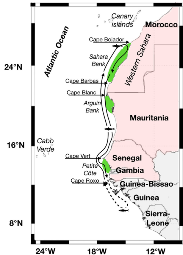
Fig. 1. Historical migration scheme for S. aurita in the sub-region (Corten et al., 2012; adapted from Boëly and Chabanne, 1978). The green shading shows the main nursery areas (Sahara Bank, Arguin Bank, and Petite Côte). The arrows show the trajectory of the large individuals suggested by fishery data analysis. The southern part of the trajectory (dotted) is not well documented and there is uncertainty on the southern limit of the migration. The countries where round sardinella constitute a large part of the fisheries catch are colored in pink. (For interpretation of the references to color in this figure legend, the reader is referred to the web version of this article.)
