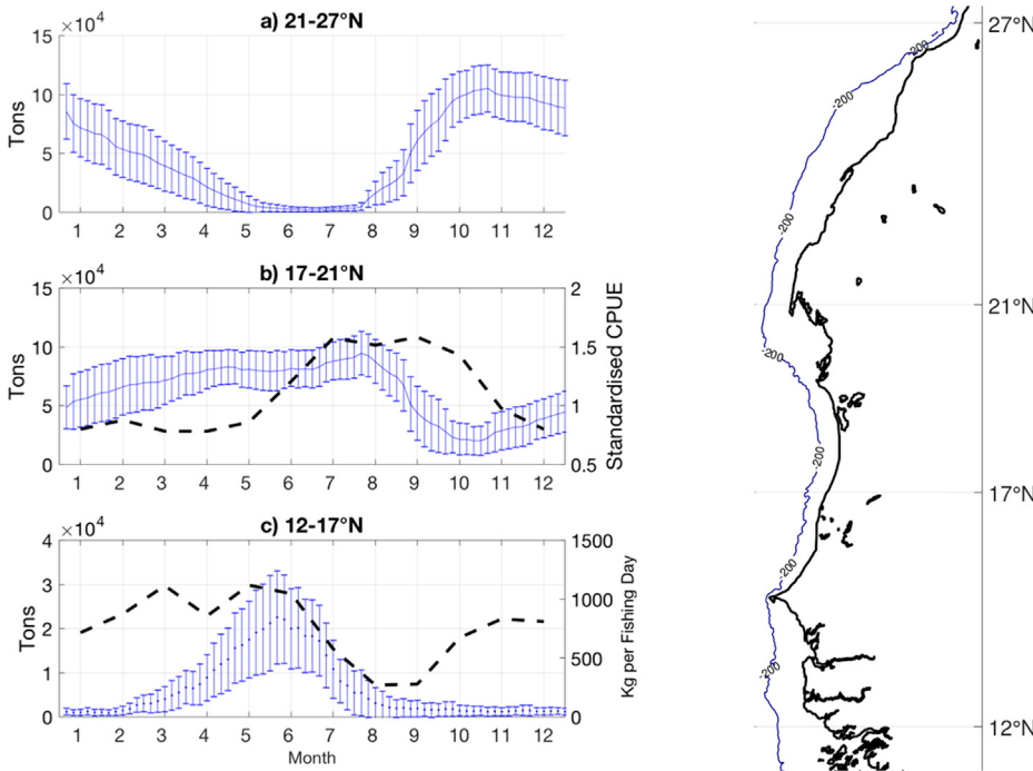
Fig. 2. Seasonal variability of round sardinella adult biomass from the model (Simulation #2, solid blue lines) and from fishery data (dashed lines). (a) Southern Morocco (no data available); (b) Mauritania (data: standardised Catch per unit effort (CPUE, IMROP, Braham et al., 2014); (c) Senegal and Gambia (data: CPUE (kg per fishing day), CRODT, Thiaw et al., 2017). The bars about the solid line indicated the range of variability of the model simulations. Note that the fishing efforts in Senegal and Mauritania refer to different types of fisheries (industrial and artisanal) so that the absolute values cannot be compared. (For interpretation of the references to color in this figure legend, the reader is referred to the web version of this article.)
