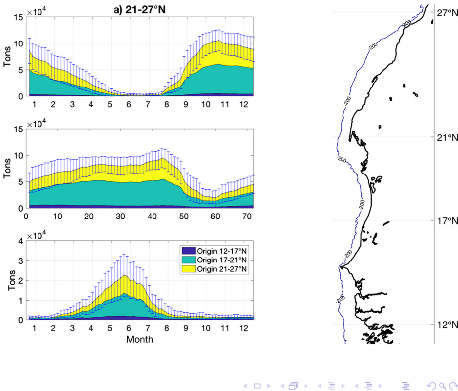
Fig. 4. Seasonal composition of round sardinella biomass reconstructed from model Simulation 2 as a function of fish origin (Table 1): Senegal and Gambia in blue (12–17°N), Mauritania in green (17–21°N) and Western Sahara in yellow (21–27°N). (For interpretation of the references to color in this figure legend, the reader is referred to the web version of this article.)
