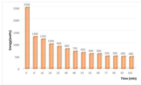
Figure 10. Energy consumption Server 1.
