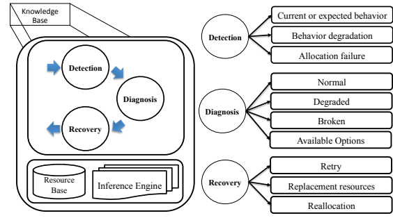
Figure 5. Scheduling Agent Behavior (General Description).
