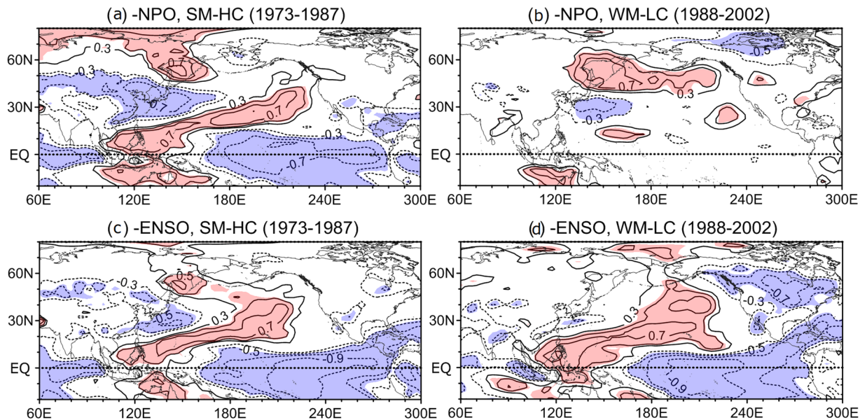
Figure 6. Maps of correlation between total precipitable water (TPW) and NPO/ENSO indices. (a,c) TPW vs - NPO and TPW vs - ENSO for 1973–1987. (b,d) Same as (a,c) but for 1988–2002. Significant correlations at the 95% confidence level are stippled in red (blue) for positive (negative) values. Adapted from Fig. 14 13 . Used with permission of American Meteorological Society.
