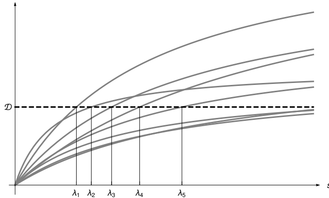
FIGURE 1. Growth functions and their break-even concentrations.
