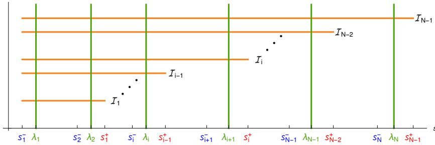
FIGURE 2. Illustration of the intervals I_i = [s_1^-, s_i^+] for i \in \{1, \dots, N-1\} (in green, the values of the break-even concentrations \lambda_i , in orange, the nested intervals I_i )
