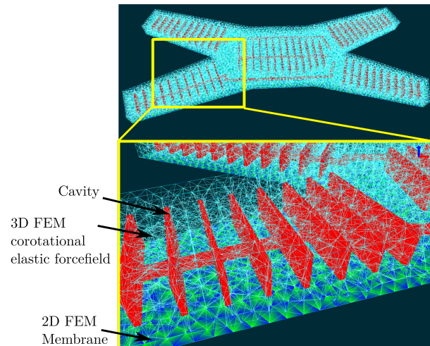
Fig. 8: Zoom in the mesh: a membrane constitutive law is applied onto the bottom layer of the soft robot. That contribution is added to the nodes located at the bottom of the robot.
