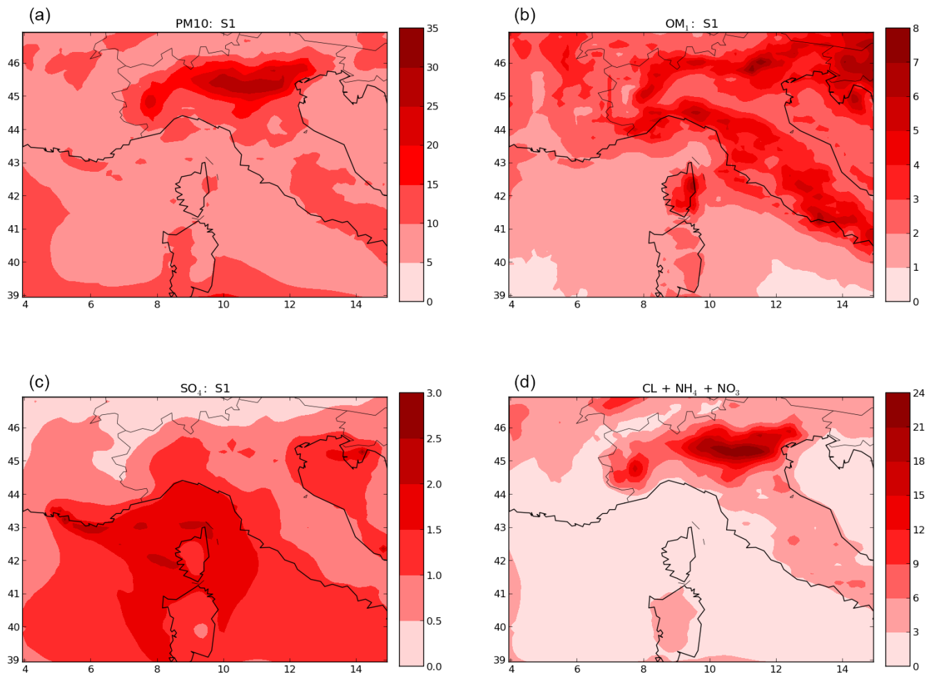
Figure D1. Maps of the concentrations of \text{PM}_{10} (a), \text{OM}_1 (b), \text{PM}_{10} sulfate (c) and other \text{PM}_{10} inorganics (nitrate + ammonium + chloride) (d) during the summer 2013 in \mu\text{g m}^{-3} .
