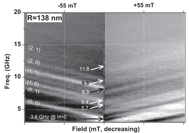
FIG. 3. Rectified voltage versus field and frequency for a nanopillar of radius 138 nm and a free layer of thickness 10.5 \text{ \AA} biased with V_{dc} = +1 \text{ mV} . The field is decreased from 110 mT (AP state) to -110 \text{ mT} . The pixelized line of color change at -1 \text{ mT} is the switching to the P state. The superimposed labels recall the proposed mode indexation. The quoted frequencies correspond to the zero field point.
