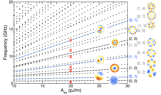
FIG. 6. Dependence of the micromagnetically calculated eigenmode frequencies (dots and lines as guide to the eye) versus exchange stiffness for circular disks of radius 138 nm, thickness 10 Å, anisotropy 0.28 \text{ MJ/m}^3 , and magnetization 0.6 MA/m, mimicking the sample on which Fig. 2 was recorded. The colored wheels illustrate the spatial profiles of each simulated mode. The red crosses are the experimentally detected frequencies.
