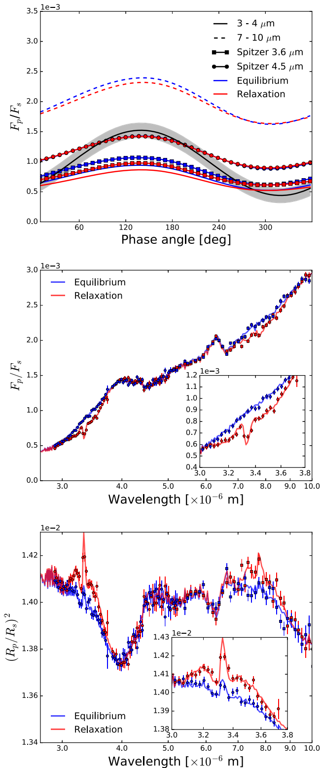
Figure 5. Top: emission phase curves in several spectral bands. The observed 4.5 \mu\text{m} Spitzer /IRAC channel curve (Zellem et al. 2014) is included (black) with 1\sigma uncertainty. Middle and bottom: secondary eclipse emission and transmission spectra with PandExo simulated observations for the NIRSPEC G395H (circles) and MIRI LRS (squares) modes, binned to a resolution of R \sim 60 and R \sim 30 , respectively.
