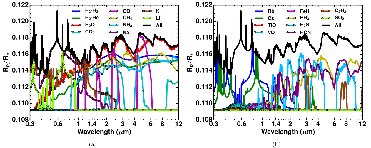
Figure A10. (a) Transmission spectra features of each individual molecule used in ATMO (1–10). \text{H}_2\text{-H}_2 (blue), \text{H}_2\text{-He} (green), \text{H}_2\text{O} (red), \text{CO}_2 (cyan), \text{CO} (magenta), \text{CH}_4 (yellow), \text{NH}_3 (light blue), \text{Na} (purple), \text{K} (brown), \text{Li} (light green) and all 20 opacities (black). (b) Transmission spectra features of each individual molecule used in ATMO (11–20). \text{Rb} (blue), \text{Cs} (green), \text{TiO} (red), \text{VO} (cyan), \text{FeH} (magenta), \text{PH}_3 (yellow), \text{H}_2\text{S} (light blue), \text{HCN} (purple), \text{C}_2\text{H}_2 (brown), \text{SO}_2 (light green) and all 20 opacities (black). No R_p/R_* offset was applied while plotting. Individual simulations are divided into blocks of 10 while plotting for clarity.
