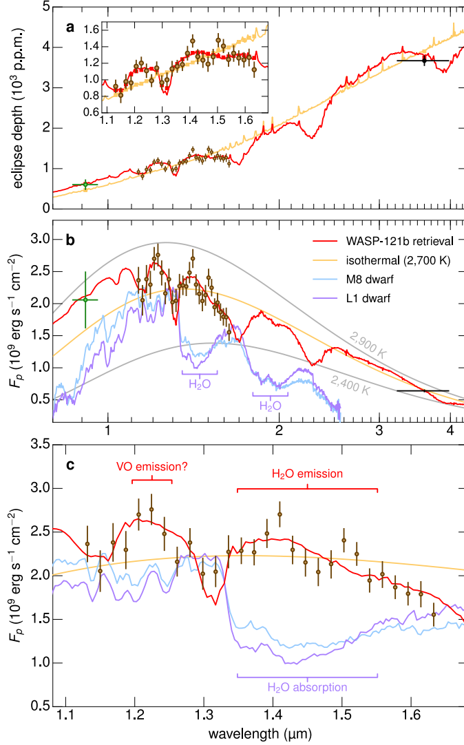
Figure 2 | Emission spectrum for WASP-121b.
