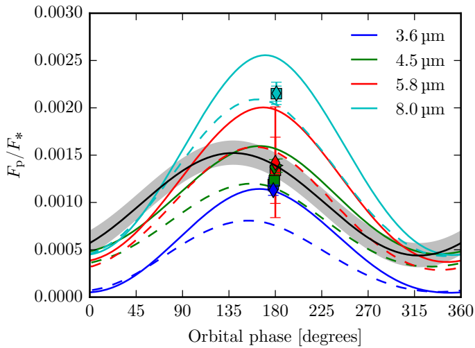
Fig. 6. Synthetic Spitzer IRAC phase curves from the Newtonian forcing model. The solid lines are calculated from the model presented in Mayne et al. (2014a) and Sect. 3 using ATM0, the dashed lines are the synthetic phase curves from Fortney et al. (2006), which are based on the models of Cooper & Showman (2005, 2006) using the same Newtonian forcing scheme. The models have been integrated over the IRAC bands using the filter functions. The data points are from Zellem et al. (2014) (►), Diamond-Lowe et al. (2014) (■) and Evans et al. (2015) (◆). The best fit to the observed 4.5 μm phase curve from Zellem et al. (2014) is shown as a solid black line, the grey shaded area is the 1σ uncertainty for the offset of the observed planet to star flux ratio.
