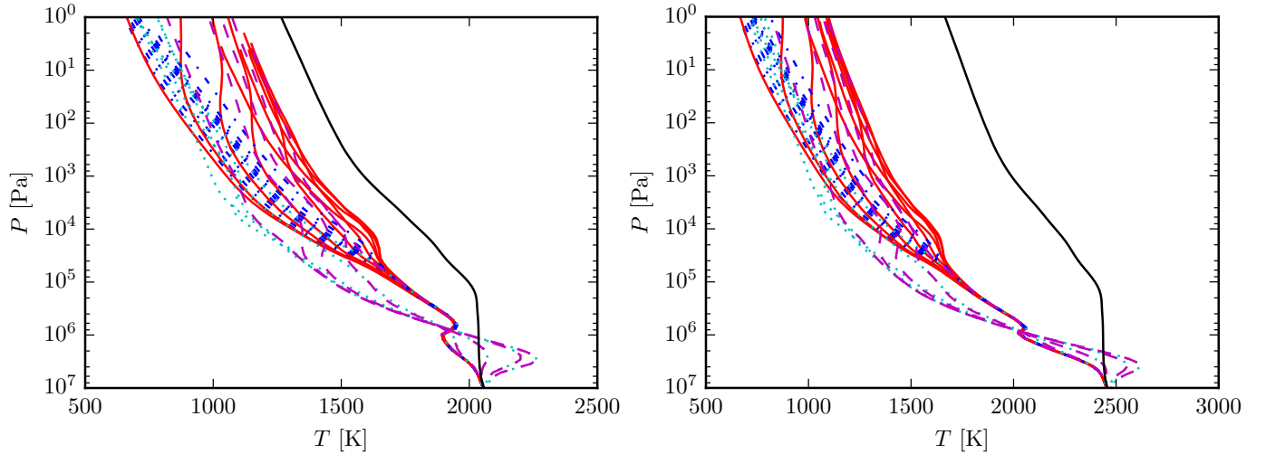
Fig. 8. P - T profiles around the globe after 1600 d for the coupled model of HD 209458b initialised with a P - T profile that is 400 K (left) and 800 K (right) hotter than the global 1D mean. Lines are as in Fig. 7.
