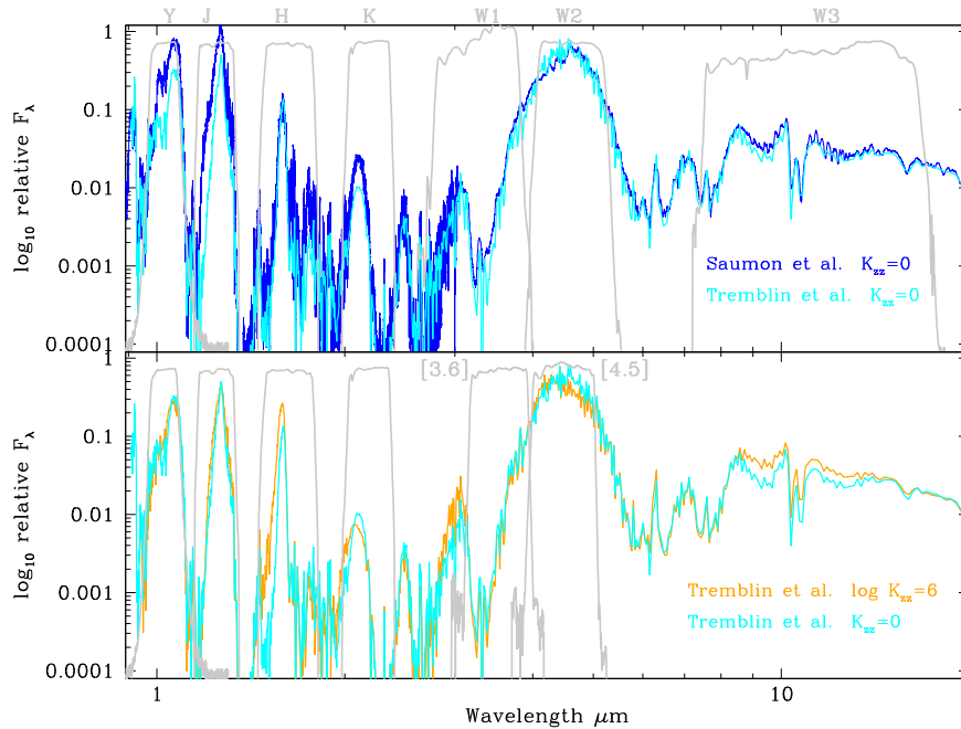
Figure 3. Comparison of Saumon et al. (2012) and Tremblin et al. (2015) cloud-free model spectra for T_{\text{eff}} = 400 K, \log g = 4.0 , solar metallicity atmospheres. The spectra have been smoothed to R \sim 1000 . Near-infrared MKO-system passbands are shown, as are the mid-infrared WISE filter passbands (upper panel) and IRAC Spitzer passbands (lower panel). The upper panel compares equilibrium-chemistry models and the lower panel compares equilibrium and non-equilibrium models. Model parameters are given in the legends. See text for discussion.
