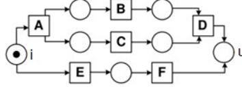
Figure 2. Process model corresponding to the modeled traces of Table 1
