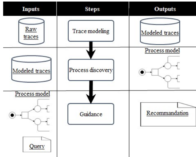
Figure 1. Process-based learning assistance method steps
