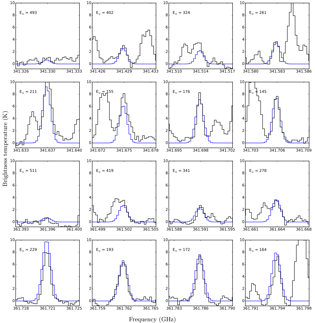
Fig. 2. Lines of \text{CH}_3\text{NC} detected in IRAS 16293B (black) overlaid with an LTE spectral model (blue). The upper energy level of each line is given in the top left corner of each plot in K.
