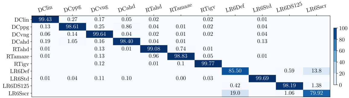
Figure 6: Confusion matrix for the supervised classification of the image processing pipeline (IPP).
