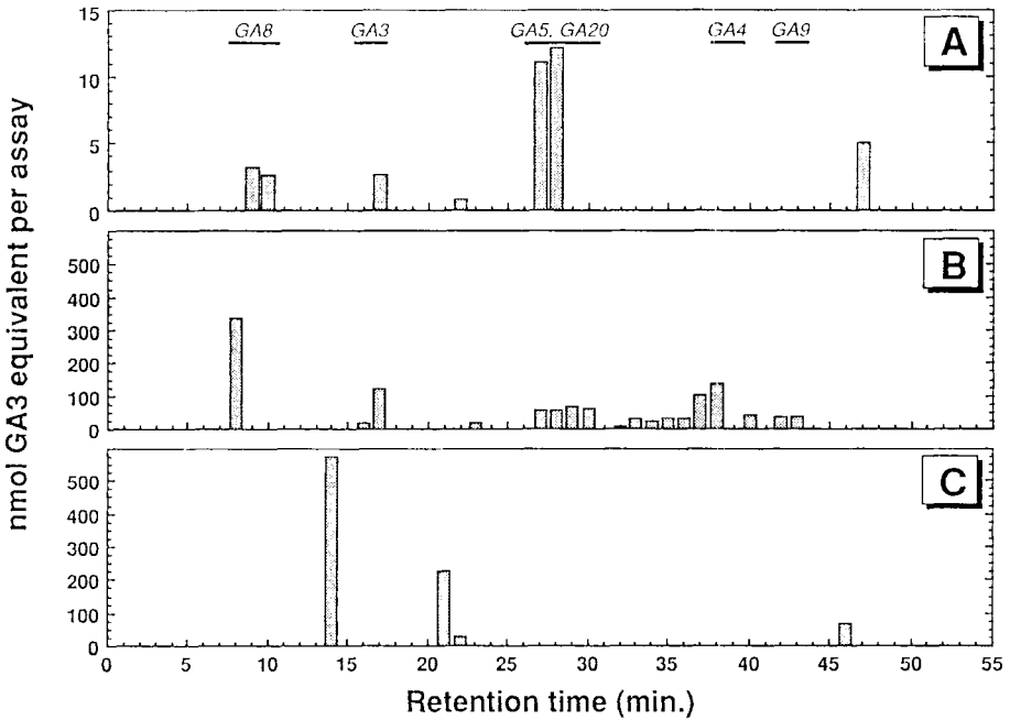
Fig. 3. Levels of GA-like compounds in purified extracts of Pseudotsuga menziesii shoots: (A: control; B: spray of GA4/7 and NAA; C: stem girdling). Extracts were chromatographed on reverse phase HPLC and activity was determined by ELISA with antiserum directed against GA3. (The scale for Y-axis is different in A, B and C.)
