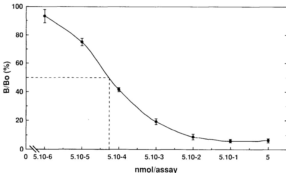
Fig. 1. Standard curve for ELISA with antiserum directed against GA3. B = binding of the tracer to the antibody in the presence of standards, and B_0 = binding of the tracer in the absence of standards.
