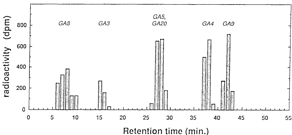
Fig. 2. Reverse phase HPLC of tritiated GAs.
