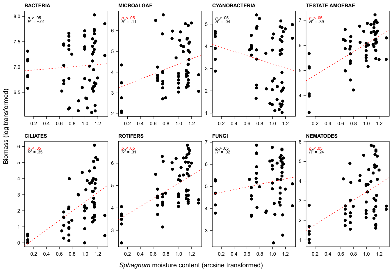
FIGURE 3 Linear regressions of the biomass of individual microbial groups to Sphagnum moisture conditions for the pooled data sets of Forbonnet and Linje peatlands
