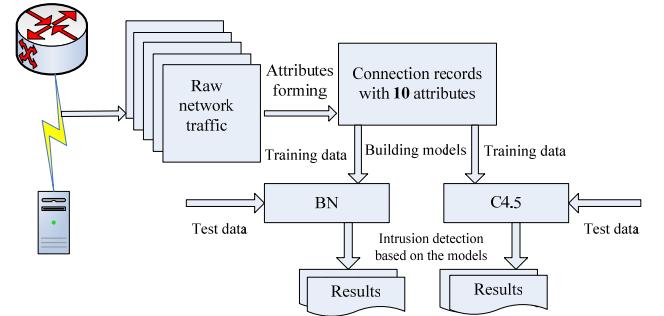
Fig. 2. Attributes selection and detection of DDoS attacks
