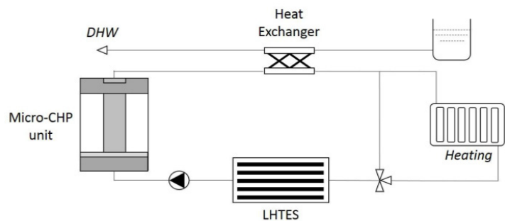
Fig. 20: Schematic view of the latent heat TES integration within the micro-CHP installation
