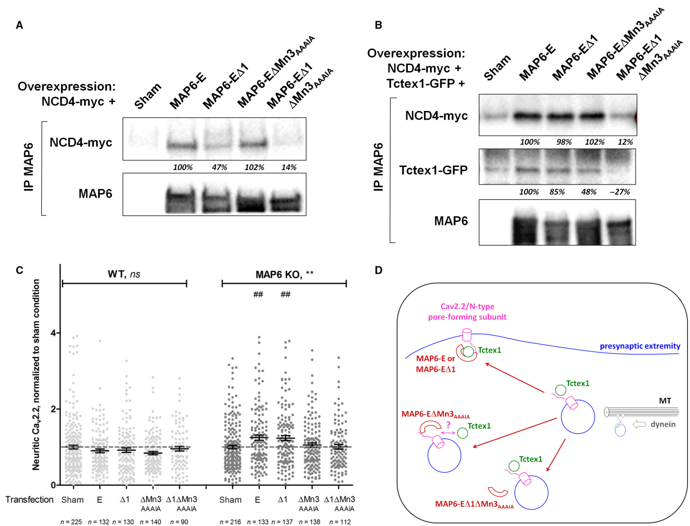
FIG. 5. Interactions of MAP6-E mutants with Ca v 2.2/N-type calcium channels and Tctex1, and restoration of neuritic content. (A) HEK-293 T17 cells were cotransfected with plasmids encoding NCD4-myc and full-length MAP6-E or mutants as in Fig. 1F. Each immunoprecipitation was performed with the anti-MAP6 23N antibody and immunorevealed by Western blotting against myc or MAP6 (23N). Note that the many MAP6 bands detected after immunoprecipitation correspond to specific degradation products as there is no signal in the sham-transfected condition. NCD4-related bands were quantified, background subtracted and normalized by that obtained with non-mutated MAP6-E (italic percentages). (B) HEK-293 T17 cells were cotransfected with plasmids encoding NCD4-myc, Tctex1-GFP and full-length MAP6-E or mutants as in Fig. 1F. Each immunoprecipitation was performed with the anti-MAP6 23N antibody and immunorevealed by Western blotting against myc, GFP or MAP6 (23N). Note that the many MAP6 bands detected after immunoprecipitation correspond to specific degradation products as there is no signal in the sham-transfected condition. NCD4-related bands and Tctex1-related bands were quantified, background subtracted and normalized by that obtained with non-mutated MAP6-E (italic percentages). (C) Quantification of neuritic Ca v 2.2/N-type calcium channels contents from WT (white discs) and MAP6 KO (grey discs) hippocampal neurons cotransfected with plasmids encoding GFP as in Fig. 4C and full-length MAP6-E or mutants as indicated, normalized by sham-transfected neurons of corresponding genotype (dashed grey line = 100%). n represents the total number of transfected neurons measured from three independent neuronal cultures. ns, not significant and **, P < 0.05, using a one-way parametric ANOVA, followed by Bonferroni's multiple comparison tests: ##, P < 0.01 as compared to sham-transfected KO. (D) Scheme of Ca v 2.2/N-type pore-forming subunit being trafficked in presynaptic extremities from vesicles moving along microtubules. When vesicles are undocked, calcium channels are not addressed to the plasma membrane in the absence of MAP6 or in the presence of the mutant MAP6-E \Delta 1 \Delta Mn3 AAAIA . In the presence of the mutant MAP6-E \Delta Mn3 AAAIA , calcium channels are not properly routed either, although MAP6-E \Delta Mn3 AAAIA retains its ability to bind the channels. Functional calcium channels are restored only in the presence of both Tctex1 and MAP6-E or mutant MAP6-E \Delta 1. [Colour figure can be viewed at wileyonlinelibrary.com ].
