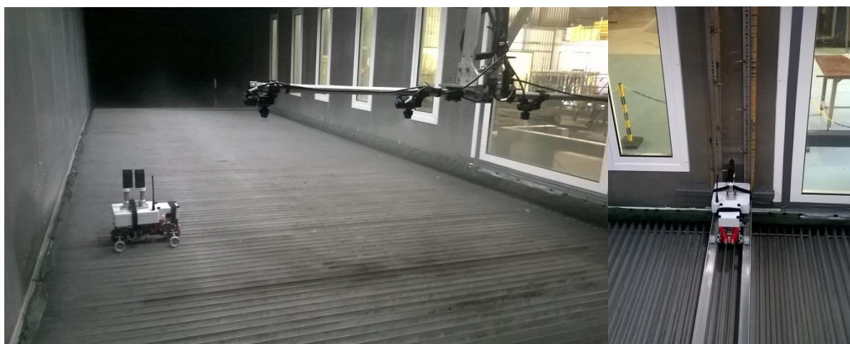
Figure 1: horizontal sampling protocol (left) and vertical sampling (right) in the wind tunnel.
